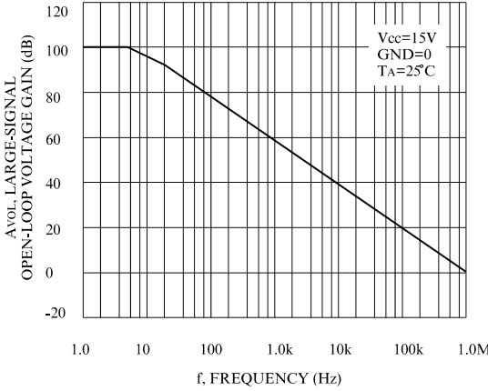
Figure 2. Open-Loop Frequency
